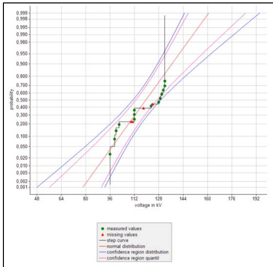
Figure 6: Evaluation of a test with continuously increasing voltage (progressiv stress) by the maximum likelihood method.
