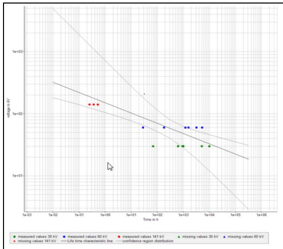
Figure 7: Lifetime characteristic with its confidence limits
