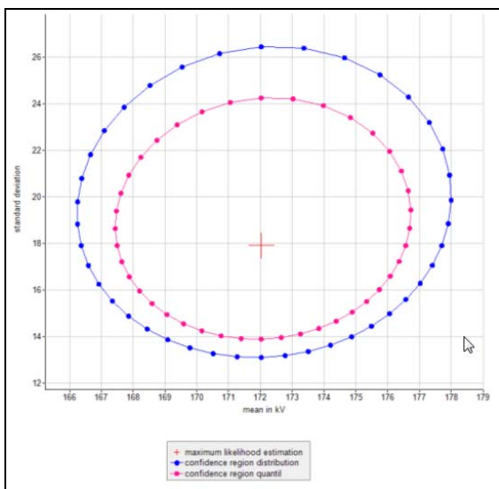
Figure 5: Regions of confidence for the quantiles and the Gauss distribution estimated according to the maximum-likelihood
