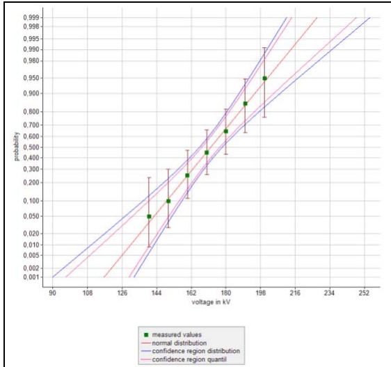
Figure 4: Evaluation of a multiple-level test by the maximum-likelihood method
