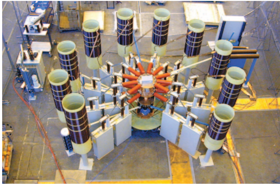
Fig. 1 1 Single-stage Impulse Current Test System with impulse energy 250 kJ, charging voltage 100 kV and max. peak current 150 kA (4/10 \mu s) with additional equipment for operating duty test
