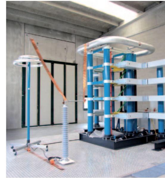
Fig. 3 Multi-stage Impulse Voltage Test System with modification to generate impulse currents
