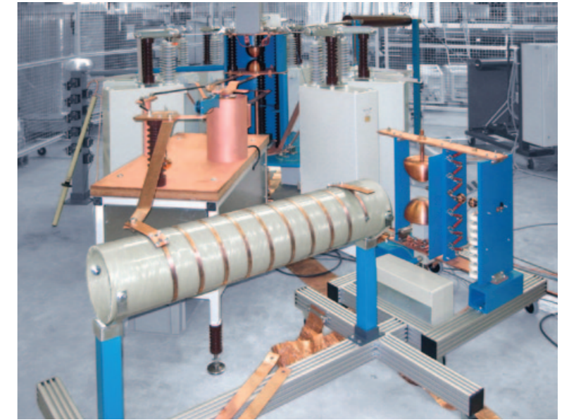
Fig. 4 Impulse Current Test System with impulse energy 128 kJ, charging voltage 80 kV and max. peak current 100 kA (10/350 \mu s) with additional crowbar circuit
