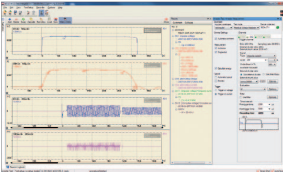
Fig. 6 Screenshot of typical residual voltage measurement
