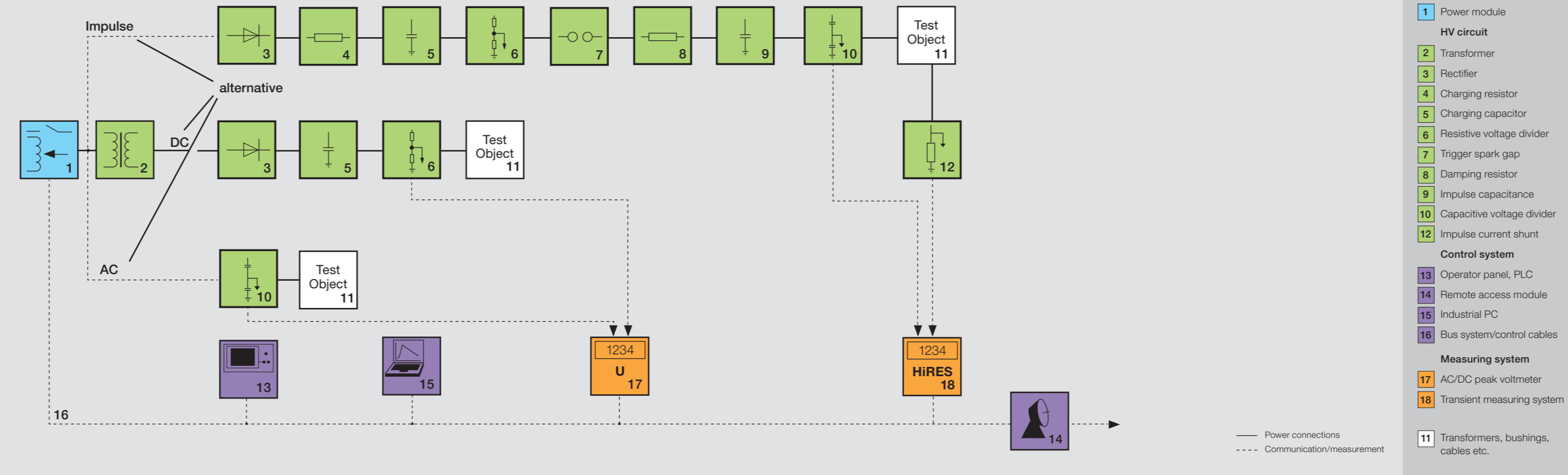
Fig. 2 Block diagram for different test set-ups as AC, DC, and impulse testing
