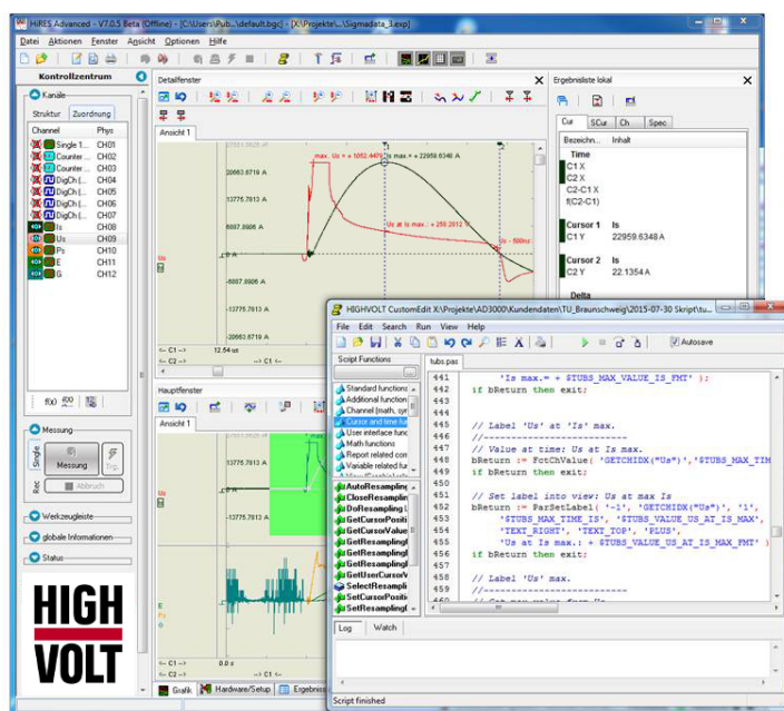
Figure 1: Function example of HiRES Advanced CustomEdit software module
